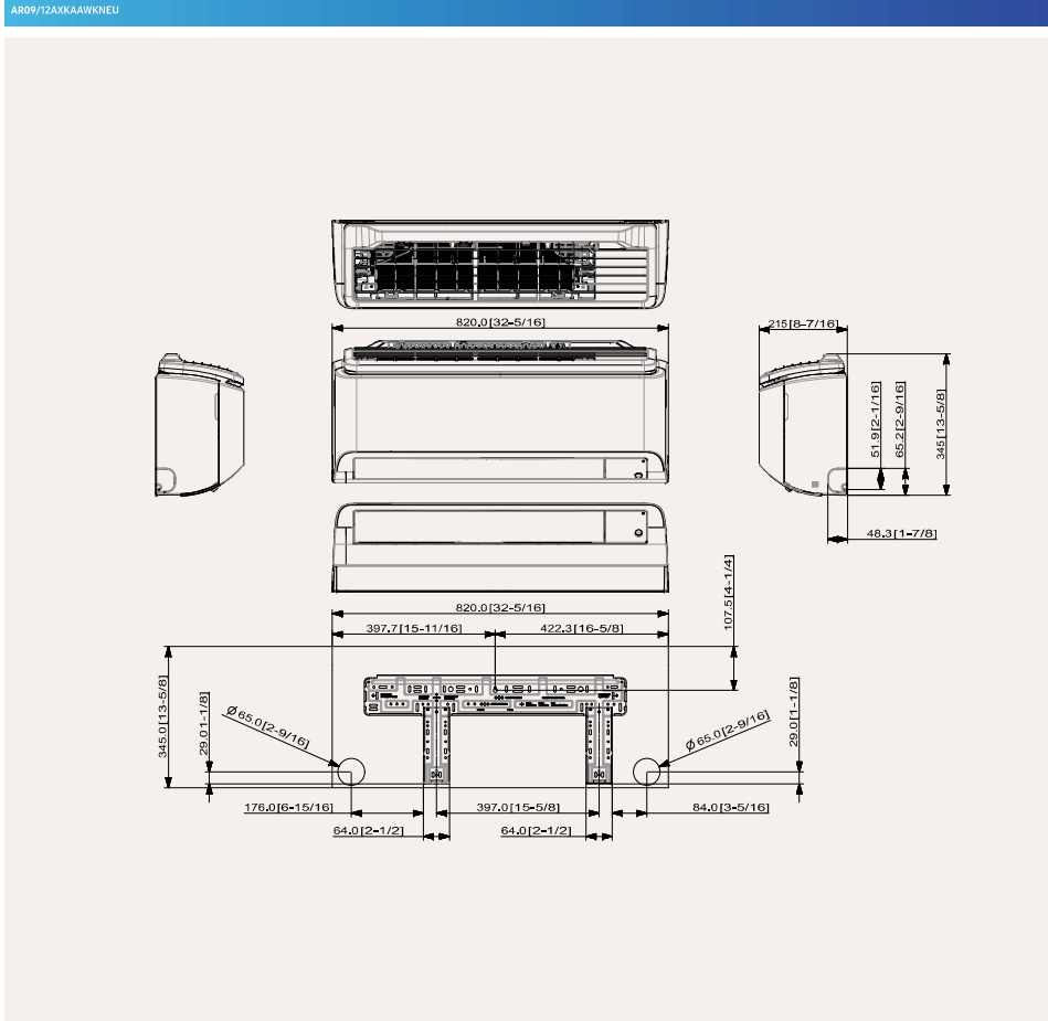
WindFree™ Pure 1.0 - Indoor
